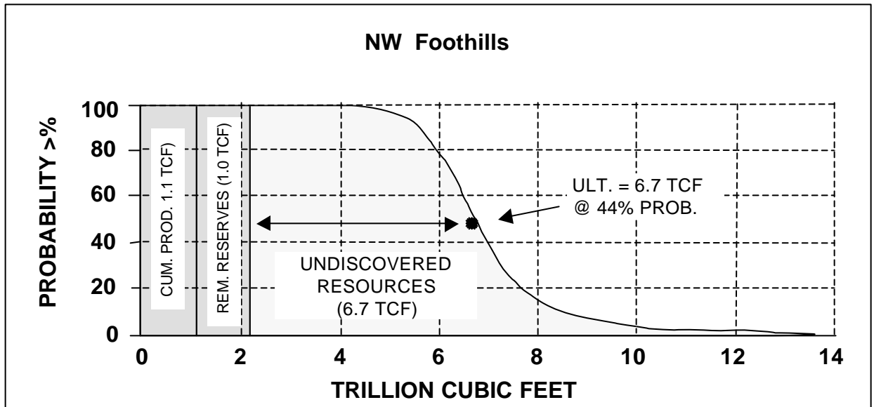
Figure 14. Distribution of ultimate marketable gas resources for the Northwest Foothills. Cumulative production and reserves to Dec. 31, 1992 (BCEMPR).
