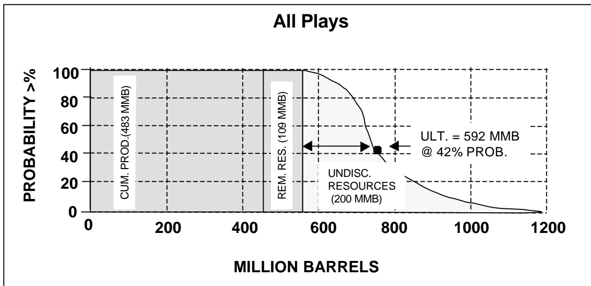
Figure 2. Distribution of ultimate recoverable oil resources. Cumulative production and reserves to Dec. 31, 1992 (BCEMPR).
