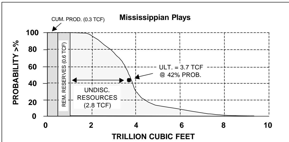
Figure 11. Distribution of ultimate marketable gas resources for the Mississippian. Cumulative production and reserves to Dec. 31, 1992 (BCEMPR).
