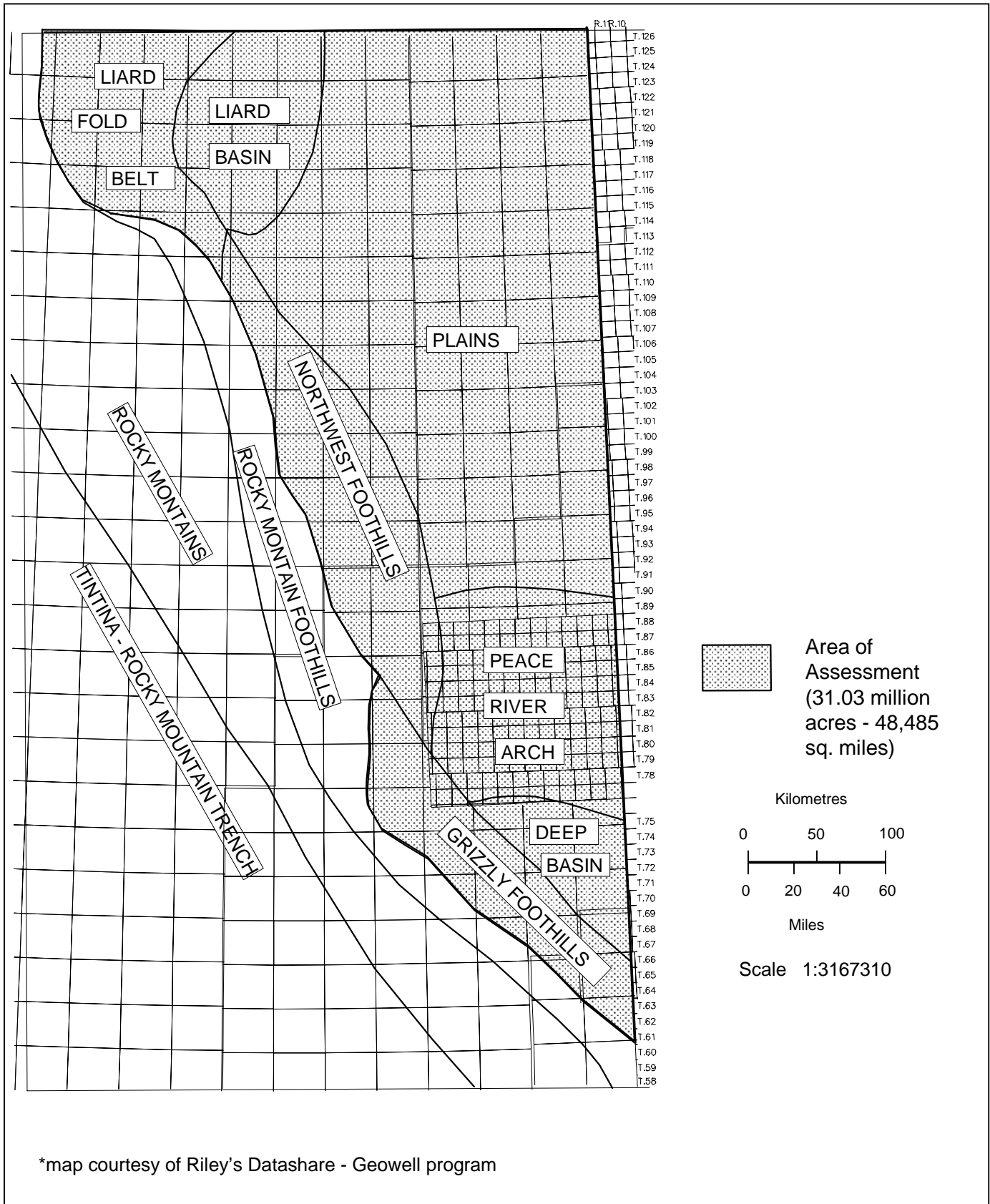
Figure 3. Generalized structural areas showing areas of assessment
