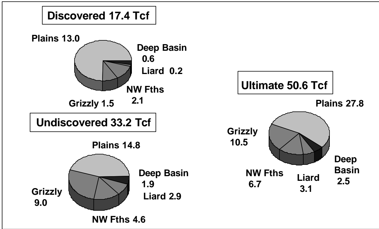
Figure 6. Distribution of gas resources by area
