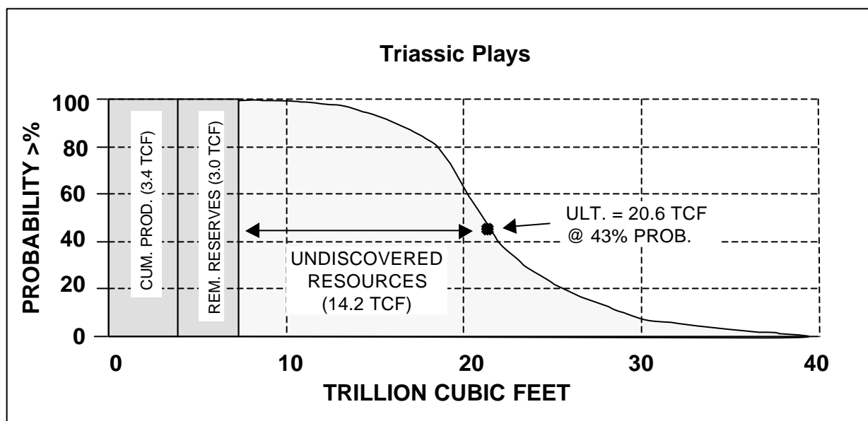
Figure 9. Distribution of ultimate marketable gas resources for the Triassic. Cumulative production and reserves to Dec. 31, 1992 (BCEMPR).
