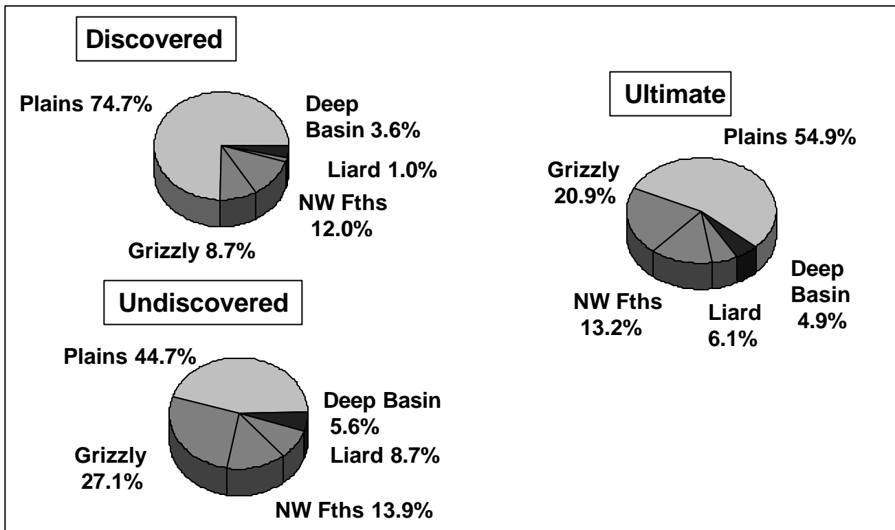
Figure 7. Percent share of gas resources by area
