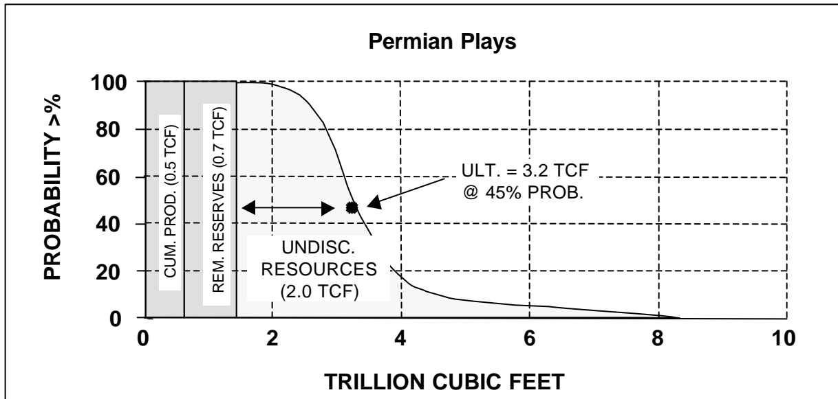
Figure 10. Distribution of ultimate marketable gas resources for the Permian. Cumulative production and reserves to Dec. 31, 1992 (BCEMPR).
