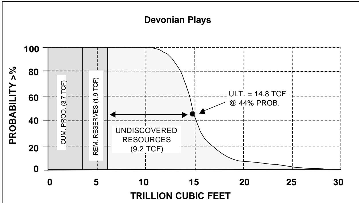
Figure 12. Distribution of ultimate marketable gas resources for the Devonian. Cumulative production and reserves to Dec. 31, 1992 (BCEMPR).
