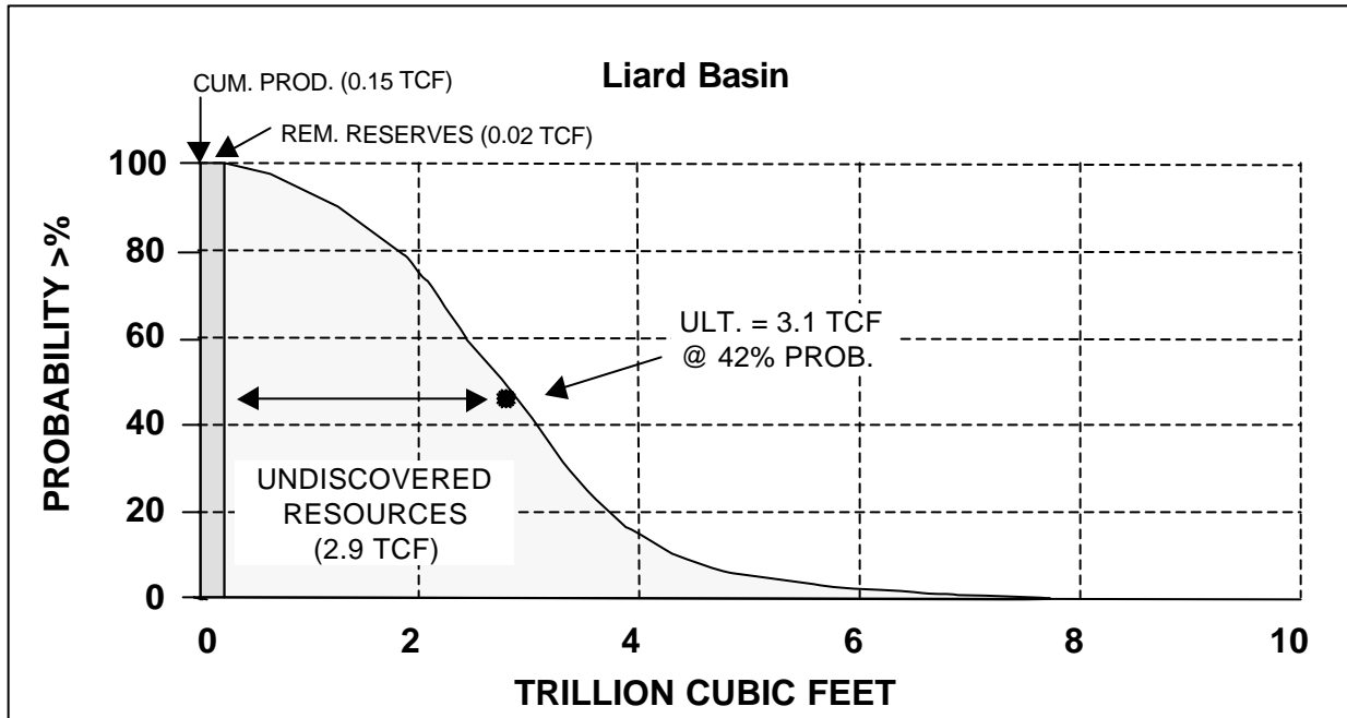
Figure 16. Distribution of ultimate marketable gas resources for the Liard Basin. Cumulative production and reserves to Dec. 31, 1992 (BCEMPR).
