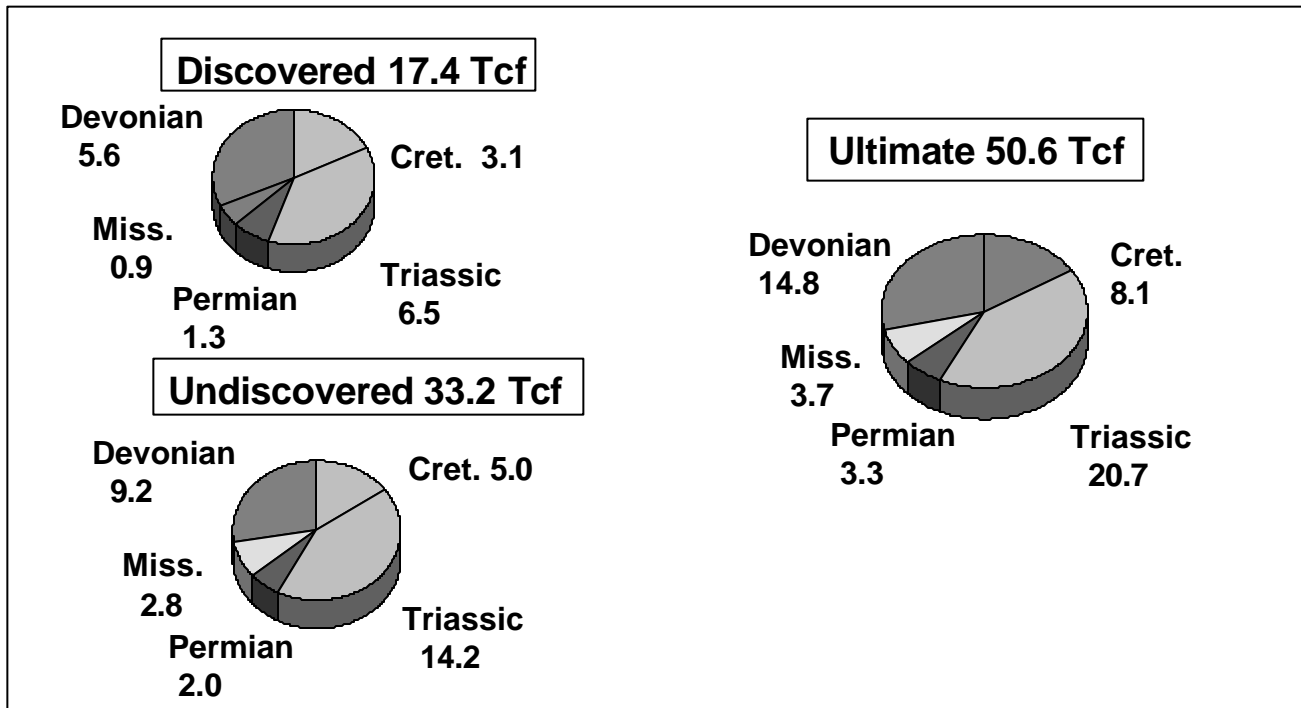
Figure 4. Distribution of gas resource volumes by geologic age
