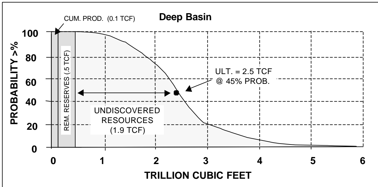
Figure 17. Distribution of ultimate marketable gas resources for the Deep Basin. Cumulative production and reserves to Dec. 31, 1992 (BCEMPR).
