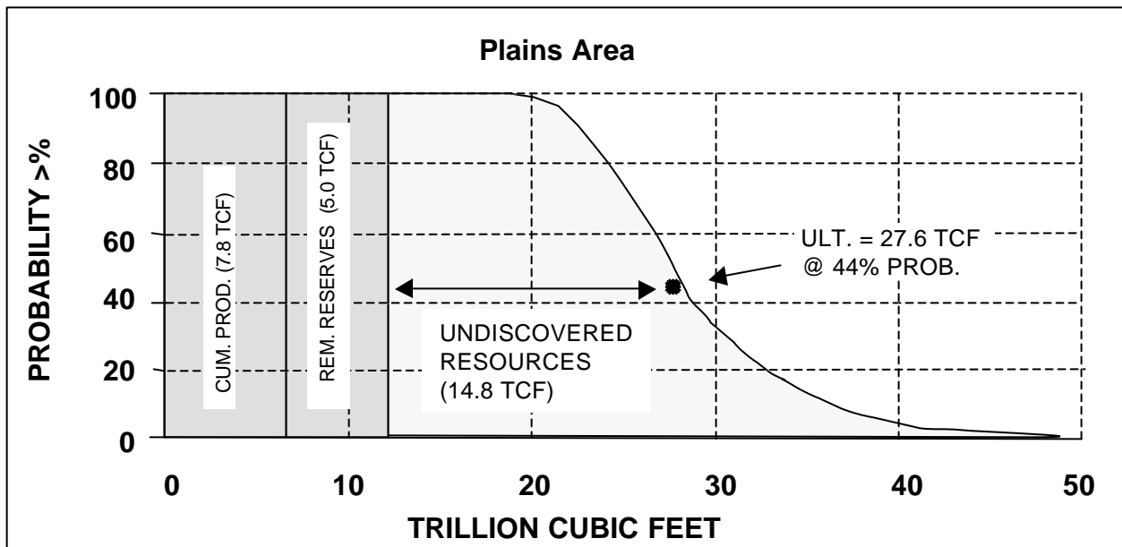
Figure 13. Distribution of ultimate marketable gas resources for the Plains area. Cumulative production and reserves to Dec. 31, 1992 (BCEMPR).
