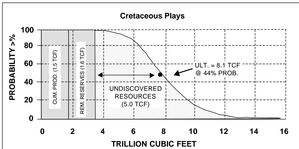
Figure 8. Distribution of ultimate marketable gas resources for the Cretaceous. Cumulative production and reserves to Dec. 31, 1992 (BCEMPR).
