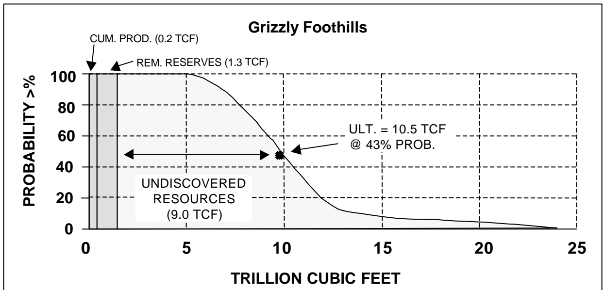
Figure 15. Distribution of ultimate marketable gas resources for the Grizzly Foothills. Cumulative production and reserves to Dec. 31, 1992 (BCEMPR).
