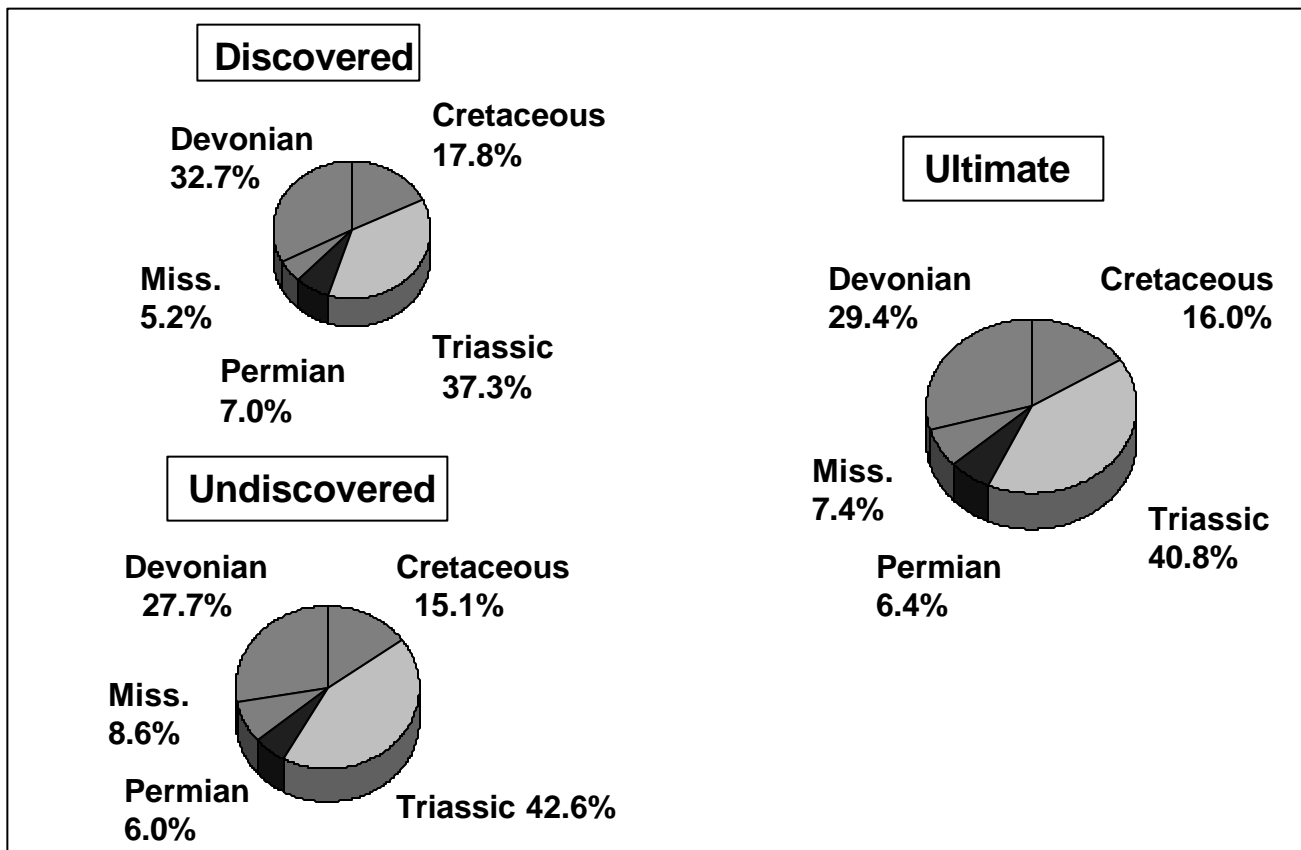
Figure 5. Percent share by geological age of gas resources
