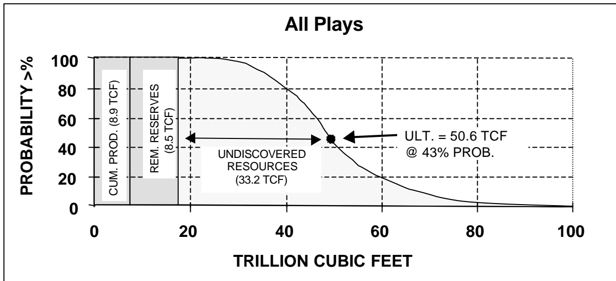
Figure 1. Distribution of ultimate marketable gas resources. Cumulative production and reserves to Dec. 31, 1992 (BCEMPR).
